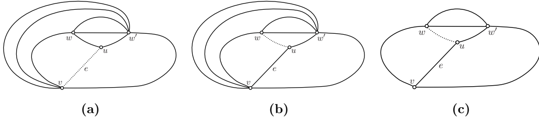
Figure 3: Contradiction to (u, v) being an edge of a segment on F'_2 in the proof of Proposition 1. Here, v \in V(F_1) , P is the only sub-segment belonging to S , and there are two segments with end vertices v and w' ; (c) is the result after the decomposition
