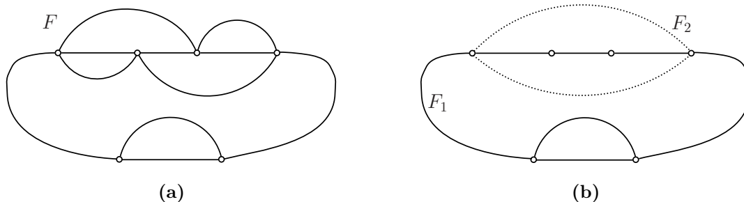
Figure 1: An example of a decomposition of F ; only the high-degree vertices are shown.
