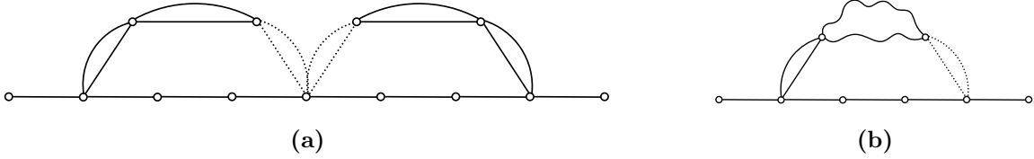
Figure 4: Examples of deletion operations on T , removing redundant double edges
