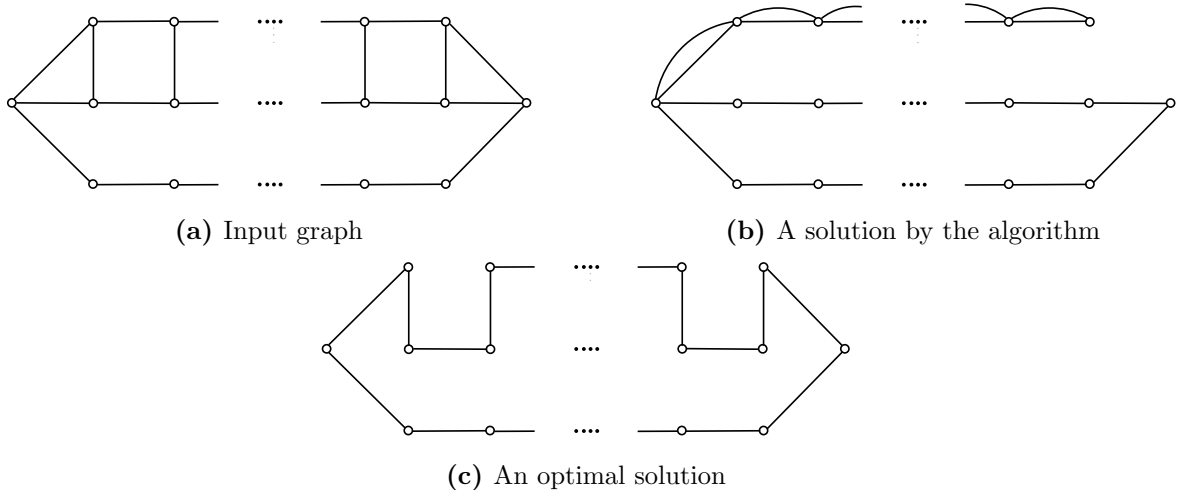
Figure 7: A tight example for the algorithm
