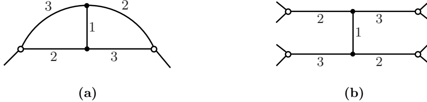
Figure 5: Modification of F'_1 so as to create three perfect matchings
