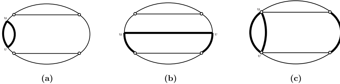
Figure 6: (a) Introduction of two new strong segments. (b) Introduction of one new strong segment and one new weak segment couple. (c) Introduction of three new strong segments, terminating one weak segment couple.
