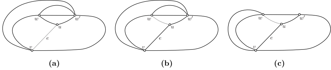
Figure 2: Contradiction to (u, v) being an edge of a segment on F'_2 in the proof of Proposition 1. Here, v \in V(F_1) , P is the only sub-segment belonging to S , and there is a single segment with end vertices v and w' ; (c) is the result after the decomposition
